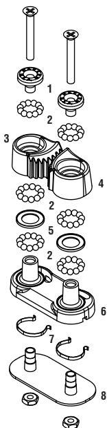
Put 11 Delrin® balls in next race.
